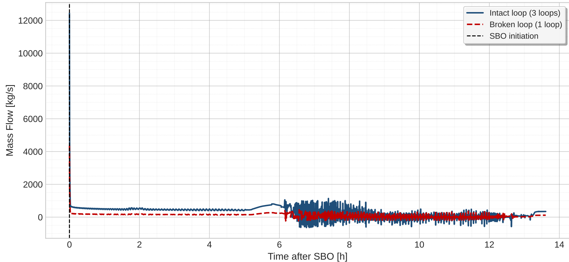
No SG Depressurization - Primary Loop Flow (Natural Circulation)
